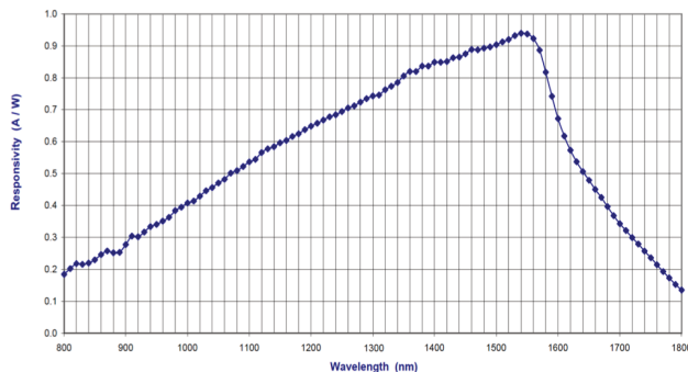
Model 271 GE Spectral Responsivity
